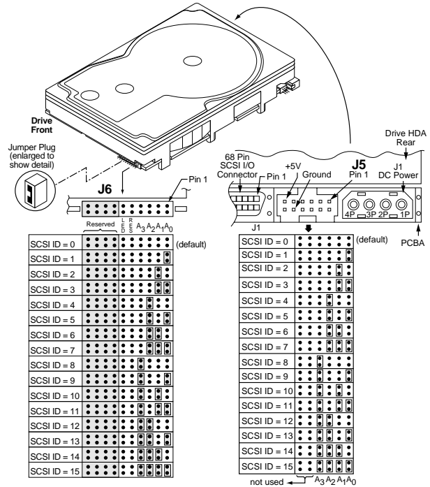
Figure 1. Setting the SCSI ID (the J5 block is on LWL/LWV models only)
