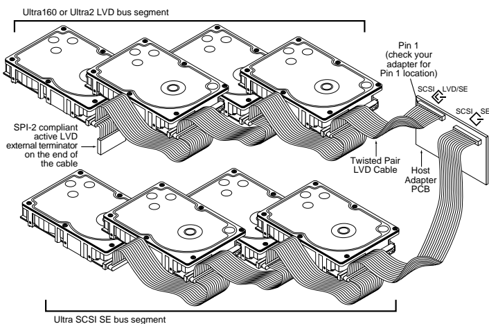
Figure 3. Cable connections and external termination
